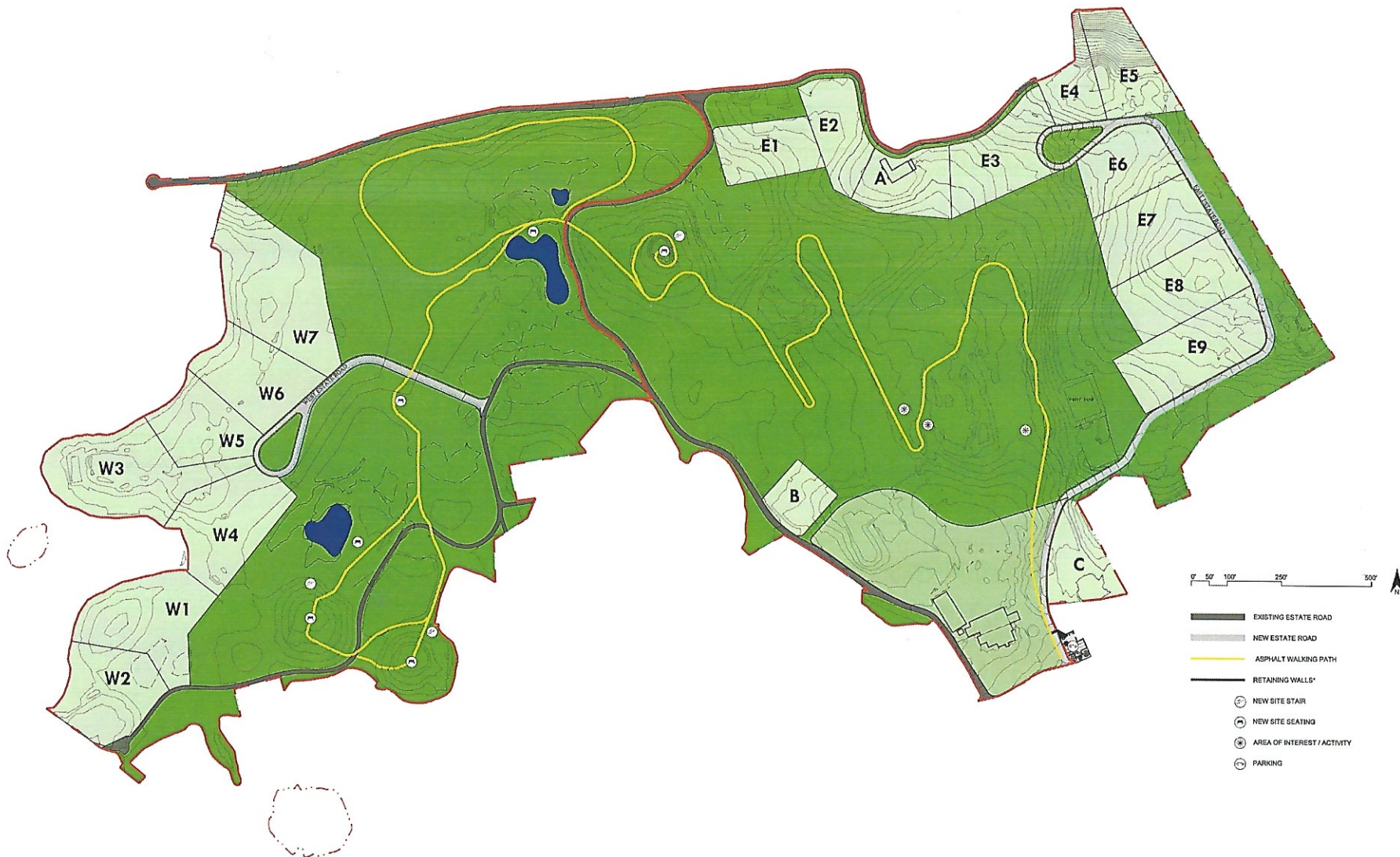
1 OVERALL SITE PLAN SCALE: 1"=133'
